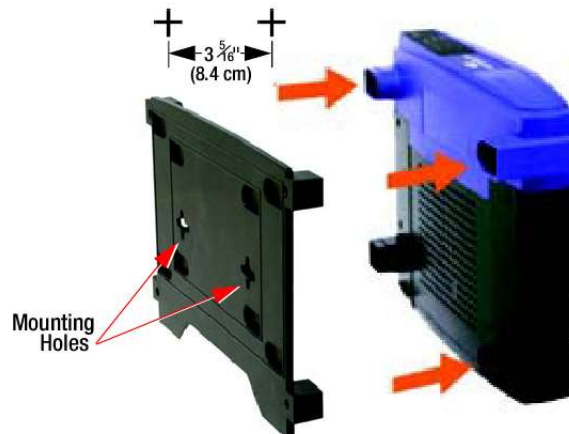
Figure 1: Wall Mounting
