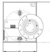
Fig. 2: Flush-mounting socket mounting and position of the regulator wheel
